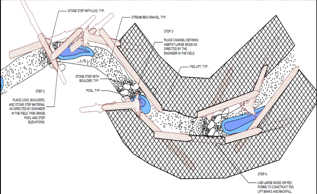
1 IKE'S CREEK TYPICAL CHANNEL SEQUENCING - PLAN VIEW
